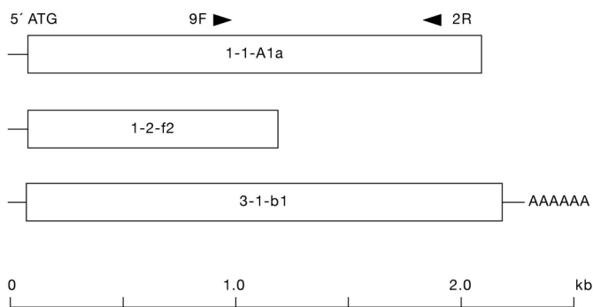
Figure 3. Schematic illustration of the three PIG11 cDNA clones isolated by immunoscreening of a cDNA expression library. The clones 1-1-A1a and 1-2-f2 are truncated versions, whereas the 3-1-b1 is full-length. The lines and boxes represent the untranslated and encoding regions, respectively. The primers, shown as arrowheads, were used to amplify a DIG-labeled probe for screening full-length cDNA clones. The sequence of the full-length cDNA clone 3-1-b1 and its putative amino acid sequence (Ms-golgin80) are provided as supplemental material.
