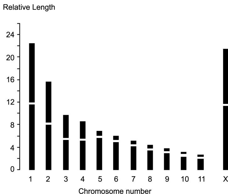
Figure 2. Idiogram of Callimenus macrogaster
